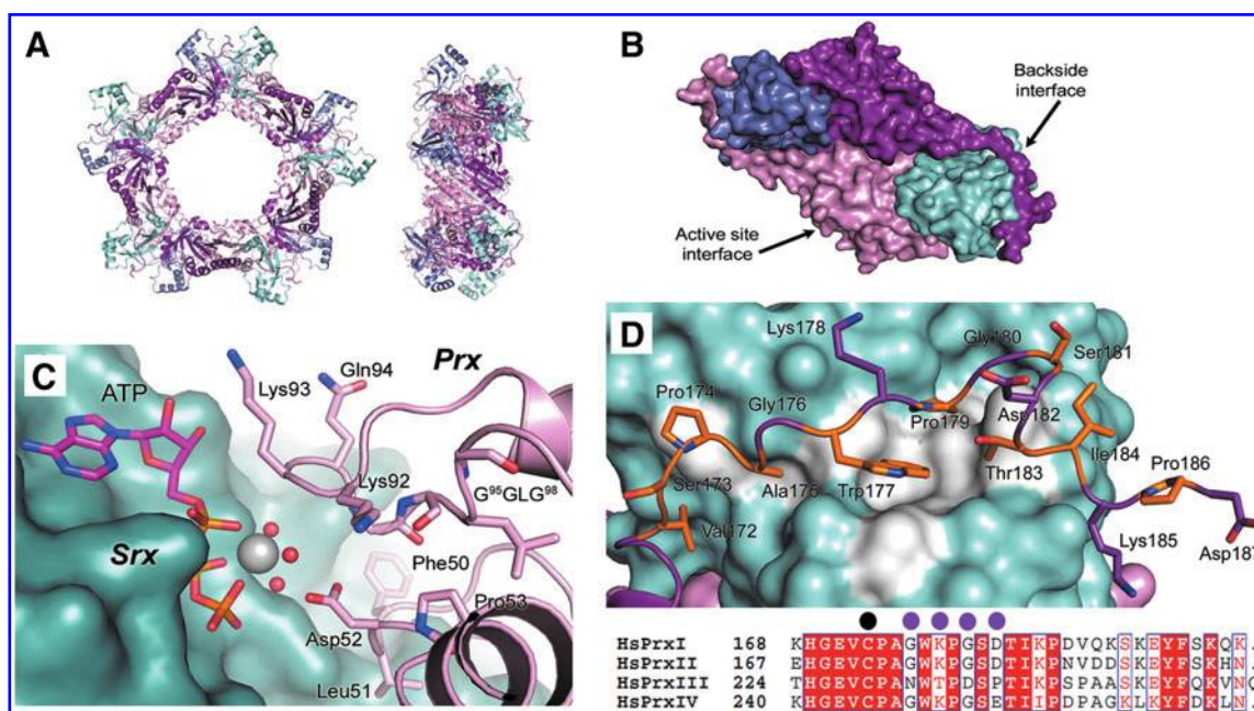
FIG. 5. The human Srx•PrxI complex. (A) Front and side views of the toroidal Srx-PrxI complex model containing 10 Prx (pink/purple) and 10 Srx molecules (blue/cyan) (28). (B) Surface representation of one Prx dimer and its active-site and backside interactions with two Srx molecules. (C) Close-up of the active-site interface in the Srx(C99A)•PrxI(C52D)•ATP•Mg 2+ complex. Same coloring scheme used as in Fig. 4B. (D) Close-up of the backside interface highlighting the local secondary structure of the PrxI C-terminus. In this complex, the resolving Cys residue, Cys 173 , was mutated to Ser, indicated by the black dot in the sequence alignment. The white surface on the Srx molecule highlights conserved residues. Orange highlighting on PrxI indicates conserved residues that interact with Srx. The purple dots on the alignment denote those residues that are different for PrxIII. (To see this illustration in color the reader is referred to the web version of this article at www.liebertonline.com/ars ).
