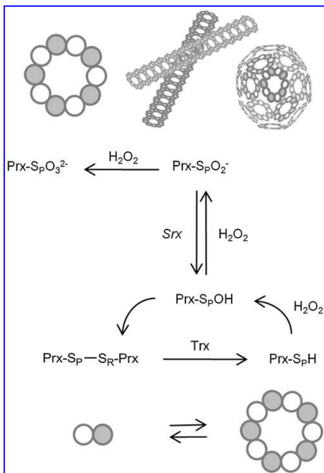
FIG. 1. Typical 2-Cys peroxiredoxin catalytic cycle and hyperoxidation. Low levels of \text{H}_2\text{O}_2 are reduced by Prx through a pair of essential Cys residues, Cys-SpH and Cys-S R H. The sulfenic acid intermediate (Cys-SpOH) reacts with the Cys-S R H residue to form an intermolecular disulfide bond, which is subsequently reduced by thioredoxin. During this process, the Prx molecules alternate between dimeric and decameric states. The reduced, decameric form of the protein is the most reactive with \text{H}_2\text{O}_2 (51, 73, 75). As the level of \text{H}_2\text{O}_2 increases, eukaryotic Prxs can react with a second \text{H}_2\text{O}_2 molecule to form the sulfinic acid form (Cys-SpO 2 - ) and, as a result, are inactivated. This hyperoxidation stabilizes the decameric state of the Prx molecule and can lead to the formation of filamentous and spherical, high-molecular-weight species; depicted schematically here. The molecular details of these interactions are unknown. Further oxidation of the Prx molecule to the Cys sulfonic acid form (Cys-SpO 3 2- ) can occur. SrX, however, can only reduce the Cys-SpO 2 - moiety.
